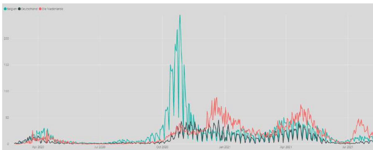
Figure 2: Covid-19, 7-day incidence for the Euregio Meuse-Rhine, March 2020 to August 2021 (Red – Dutch area, green – Belgian area, black – German area).
