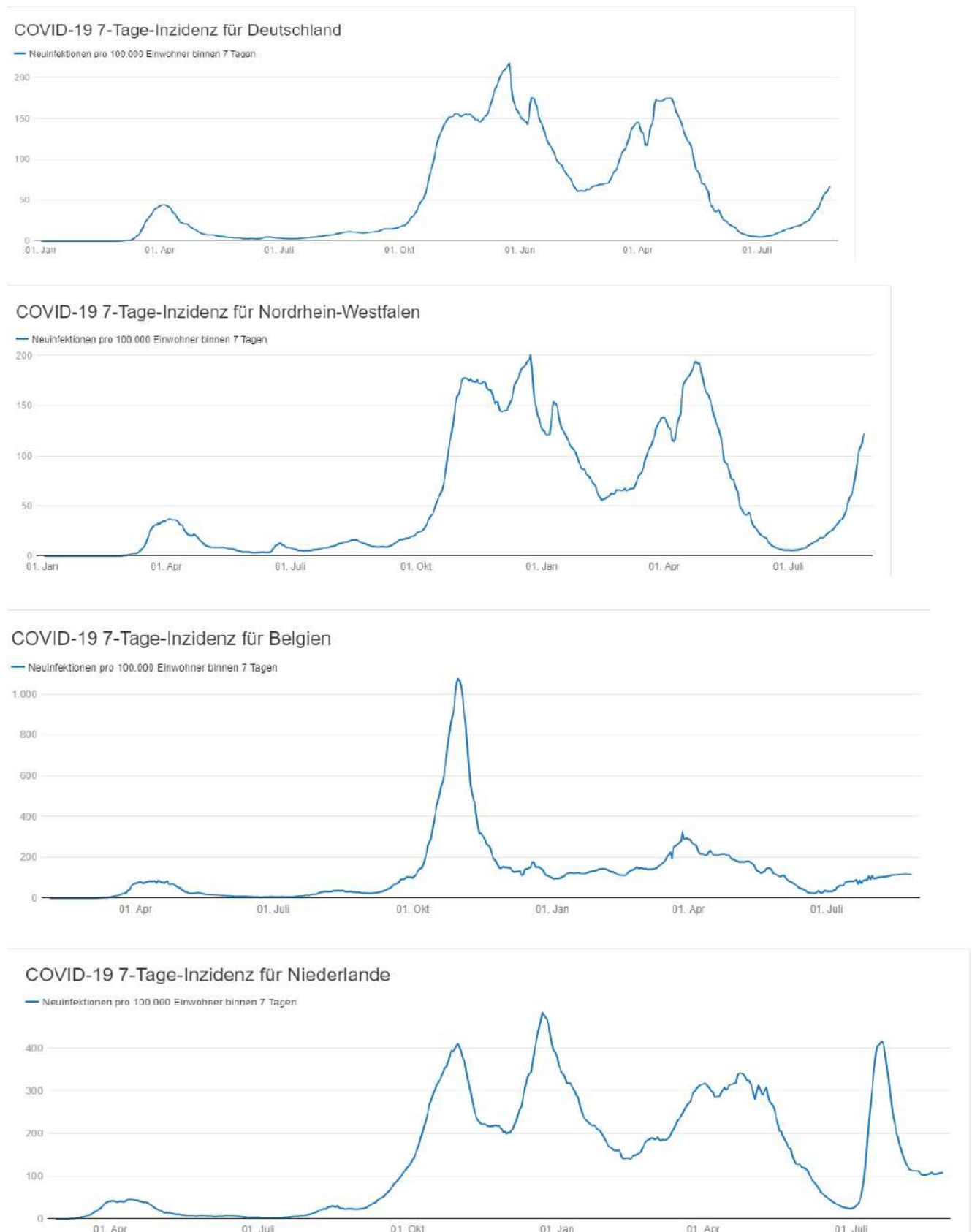
Figure 3: Covid-19, 7-days incidences for Germany, NRW, Belgium and the Netherlands from January 2020 until August 2021
